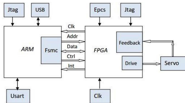
Figure 4. Main structure of the controller [12]
