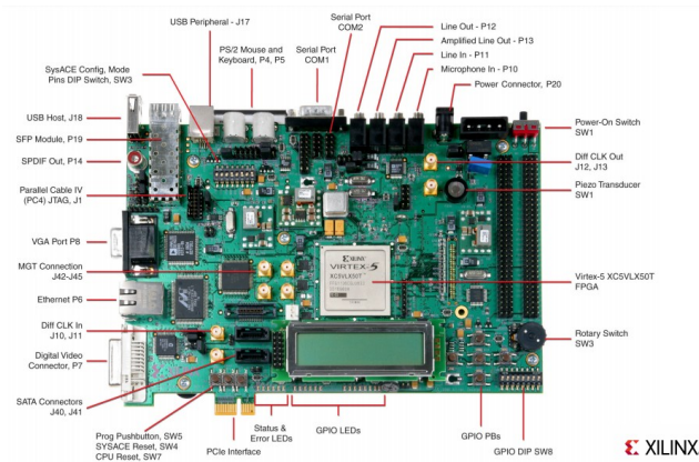
Figure 2. Xilinx board Virtex5 ML505 [11]
