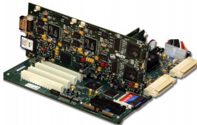
Figure 5. View of the BioServer device [13-14]
