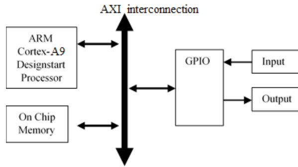
Figure 8. Block diagram of the ARM processor system
