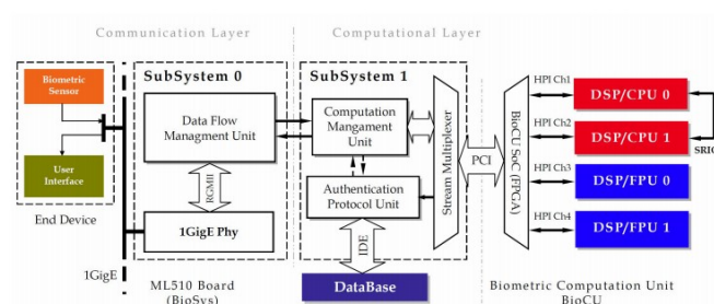
Figure 6. Block diagram of the BioServer device [13-14]
