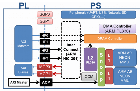
Figure 7. Architecture of a Xilinx ZYNQ board [15]
