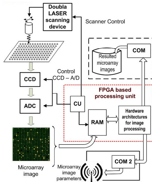
Figure 3. System design block diagram for [10]
